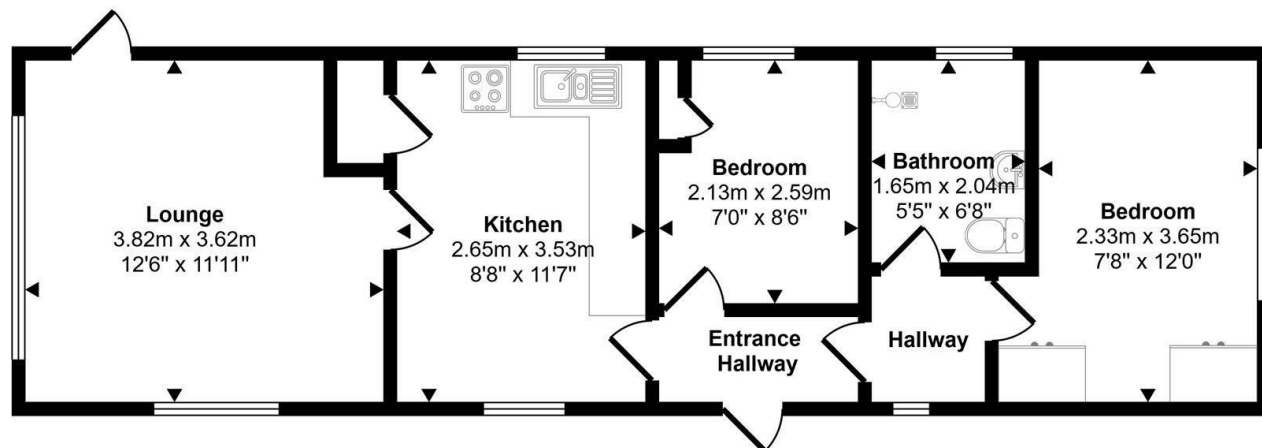
Floorplan
